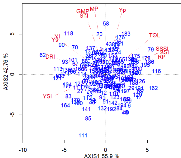
Figure 4. Genotype \times index (GI) biplot of durum wheat landraces and calculated drought tolerance indices. Yp: Grain yield under irrigated condition, Ys: Grain yield under rainfed condition, TOL: Tolerance index, MP: Mean productivity, GMP: Geometric mean productivity, STI: Stress tolerance index, SSI: Stress susceptibility index, SSSI: Schneider's Stress Severity Index, YSI: Yield stability index, YI: Yield index, DRI: Drought response index, RP%: Yield reduction percentage
