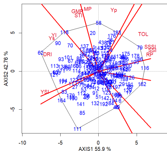
Figure 4. The polygon view of genotype \times index (GI) biplot of durum wheat landraces and calculated drought tolerance indices
