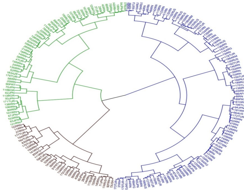
Figure 8. Cluster analysis of durum wheat landraces based on grain yield and drought tolerance indicis. Clusters 1, 2 and 3 are marked in green, purple, and brown, respectively.
