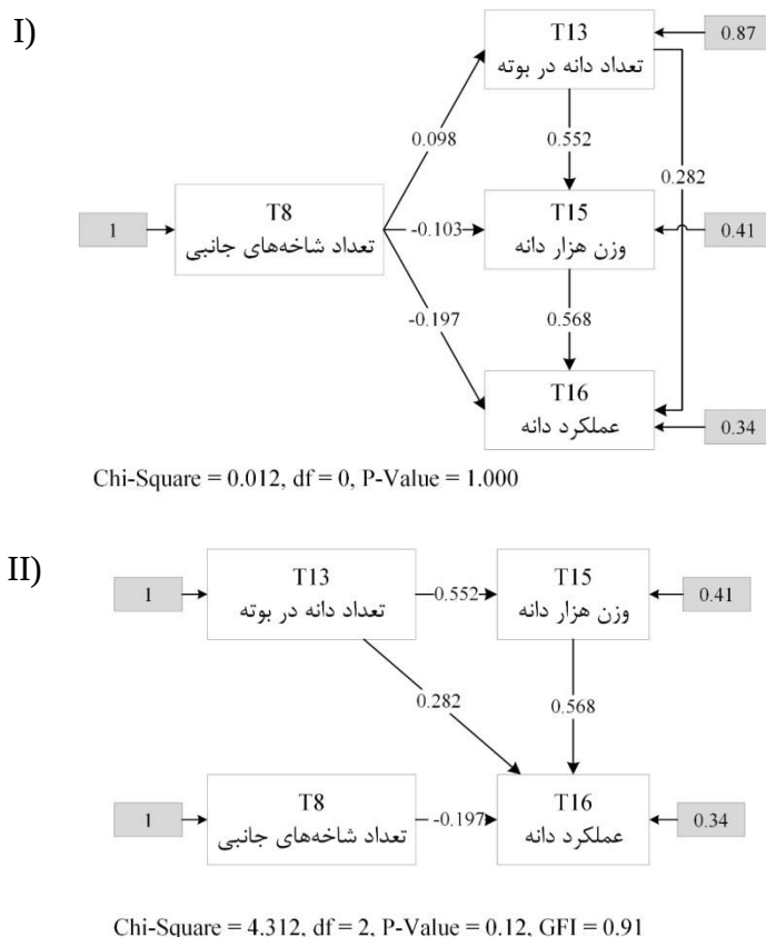
Figure 1. The diagram of path analysis of four traits entered in model based on I) the just identified model and II) the over-identified model
