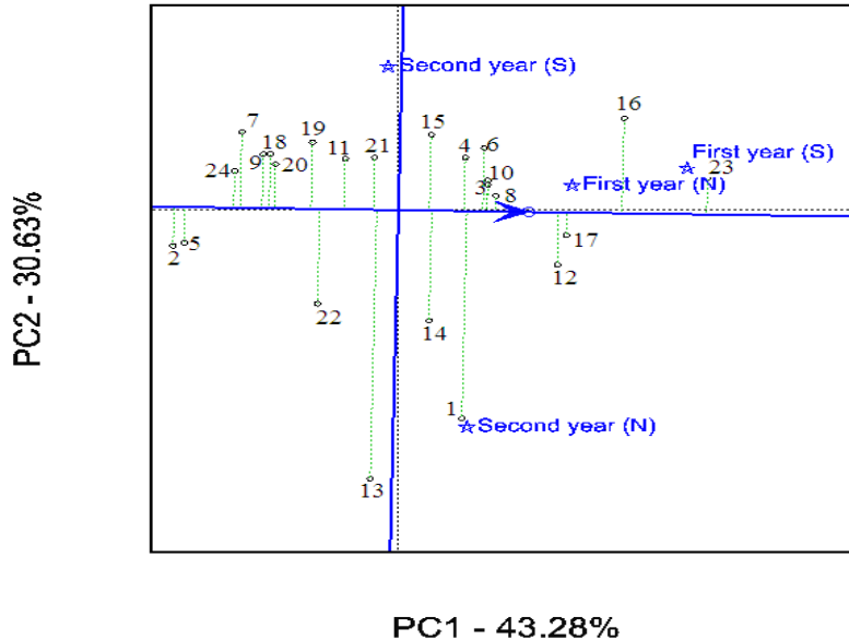
Ranking biplot (Total - 73.91%)
