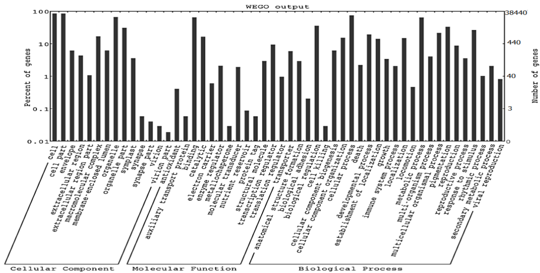
Figure 5. Functional classification of assembled unigenes containing microsatellites. Each bar represents the percentage of unigenes match to each GO term. Plot with Y axis is in log (10) scale
